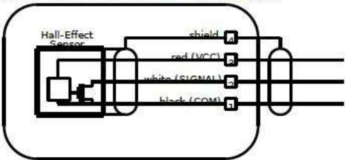
HTM TURBINE METER TERMINALS
